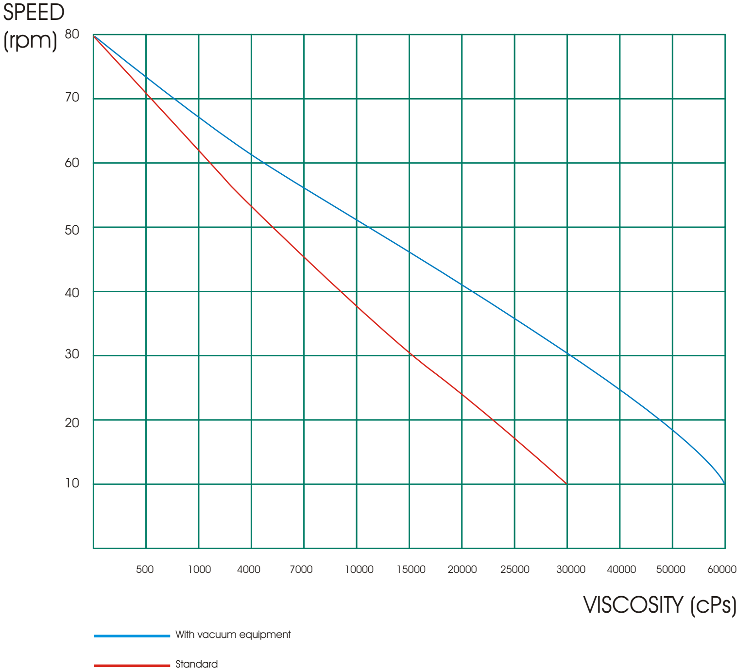
Viscosity Curve
